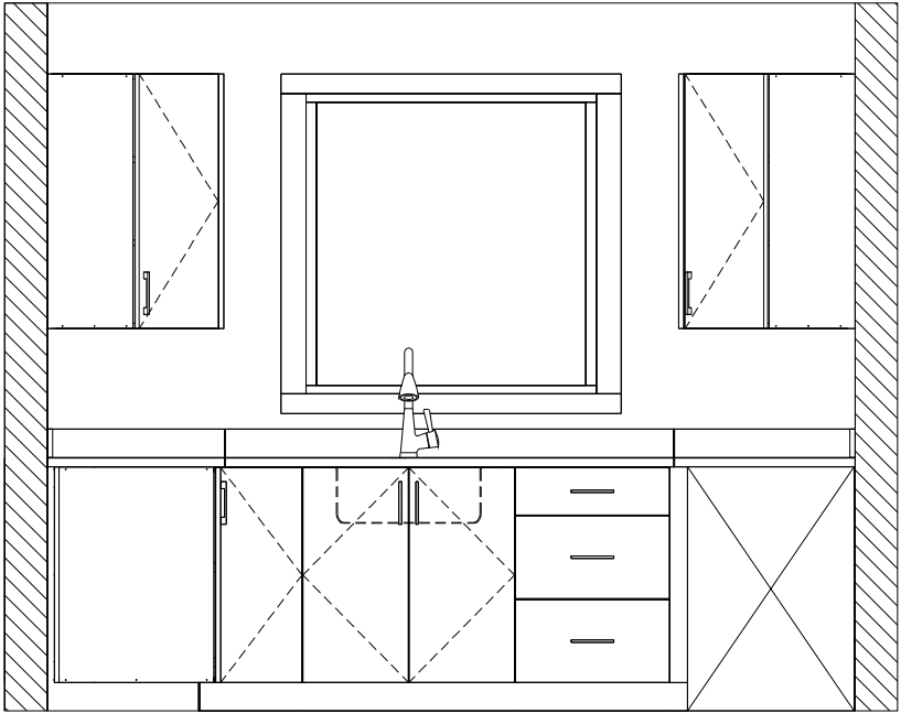
KITCHEN ELEVATION
