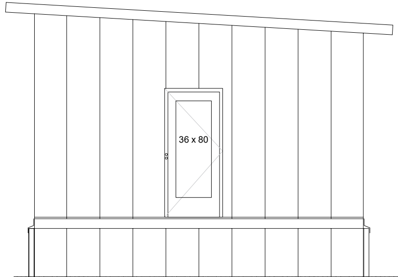
STUDIO WEST ELEVATION
