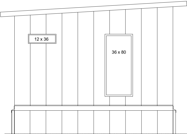
STUDIO EAST ELEVATION
