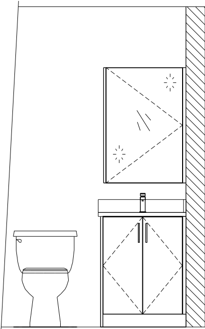
VANITY ELEVATION
