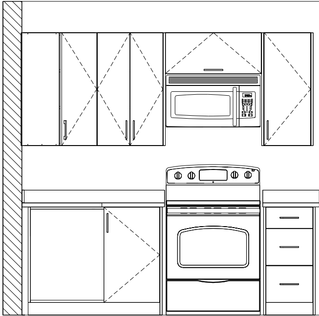
KITCHEN ELEVATION
