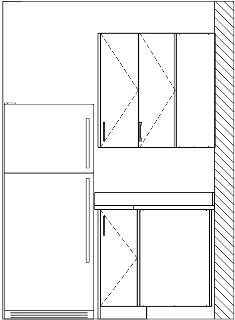
KITCHEN ELEVATION
