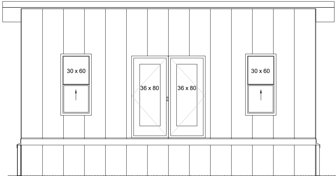
STUDIO - 1 BEDROOM NORTH ELEVATION
